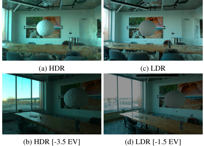
Figure 5: HDR Volumetric Radiance Map. The diffuse sphere is rendered using our hybrid algorithm. Images rendered using the NeRF trained in 32-bit HDR (a, b) achieve a higher level of lighting realism than those rendered with 8-bit LDR (c, d).
