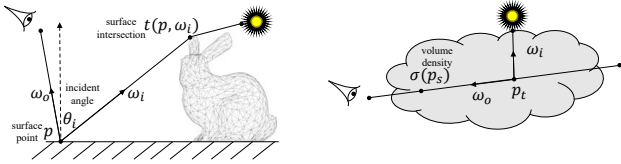
Figure 2: Light transport on the surface ( left ) and in the medium ( right ).
