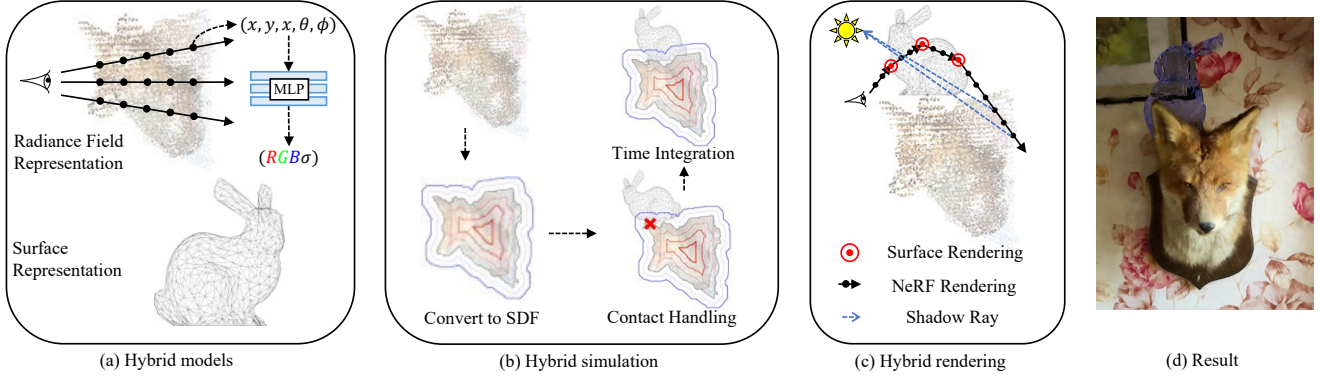
Figure 3: Pipeline overview. Our method takes an optimized radiance field model and surface meshes as inputs. We can run a physics simulation between the NeRF and meshes. The updated mesh vertices and NeRF transformations are synchronized to the renderer, which uses Monte Carlo simulation to sample ray paths. As the ray travels through space, it alternates between surface rendering (ray-tracing) and NeRF rendering (ray-marching), both updating its radiance.
