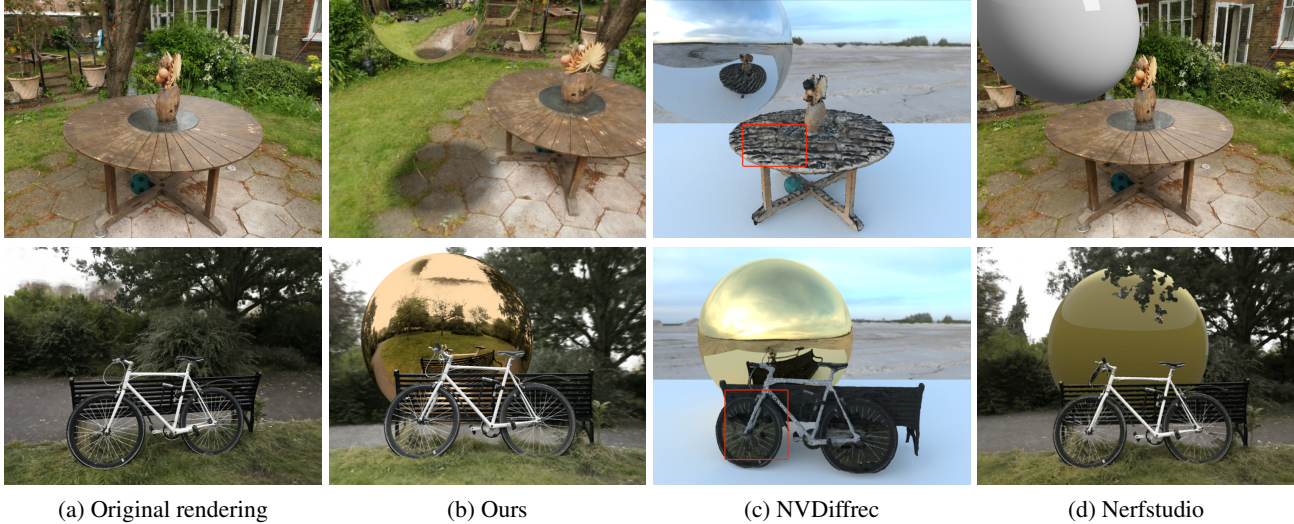
Figure 6: Rendering comparison for virtual object insertion. We insert a reflective metal ball into the Garden and Bicycle scenes from the Mip-NeRF 360 dataset [5]. (b) Our hybrid method produces results of superior visual quality with fewer artifacts. (c) We extract the foreground mesh using NVDiffRec, then insert the synthetic ball and render using ray tracing. Extracting an explicit mesh object results in noticeable artifacts such as the noisy table surface, and missing thin structures like the bicycle’s wheel and the bench. (d) The 2D compositing workflow of Nerfstudio suffers from non-3D-aware occlusion masks and a limited ability to accommodate realistic interreflection.
