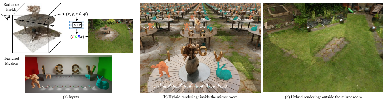
Figure 1: Mesh-aware rendering of radiance fields. We place a cubic mesh with reflective textures and other synthetic mesh objects in the MipNeRF-360 Garden [5] scene. Our mesh-aware rendering explicitly computes the rays bouncing inside the mirror room, creating an ‘infinite mirror room’ visual effect.
