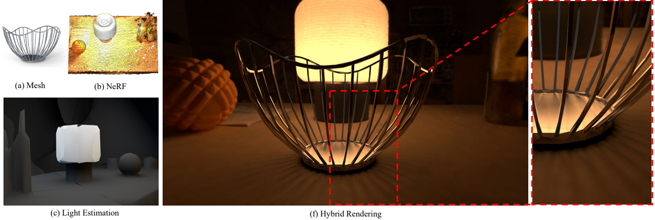
Figure 4: Shadow Casting. We estimate the geometry and light source of the scene and insert a metal basket onto the desk. Our pipeline can render the realistic reflection and shadow effects caused by the synthetic mesh.
