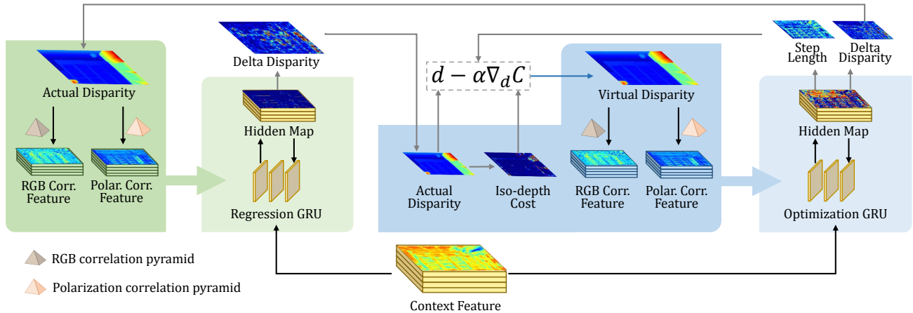
Figure 2. The hybrid GRU-based update operator is shown in this figure to interpret how multi-domain correlation features and iso-depth cost are processed and fused. The cascaded dual-GRU architecture consists of a regression GRU that provides an initial disparity prediction and an optimization GRU that further refines the disparity.
