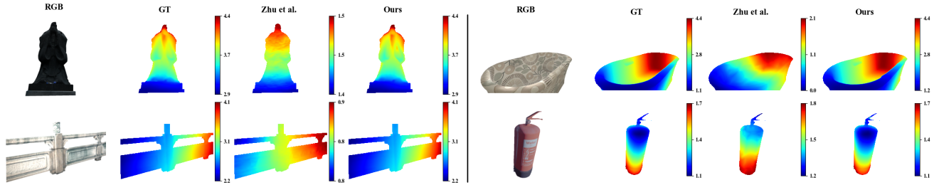
Figure 5. Qualitative results of our DPS-Net and traditional polarimetric method [51]. The RPS dataset examples are exhibited on the left, and the IPS dataset examples are displayed on the right. Each image has a respective color bar depending on the depth range of the depth image. Our results fit with the ground truth well. The predictions of [51] have consistent variation but different ranges with ground truth.
