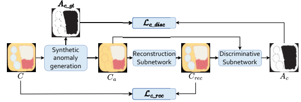
Figure 3. Composition branch architecture.
