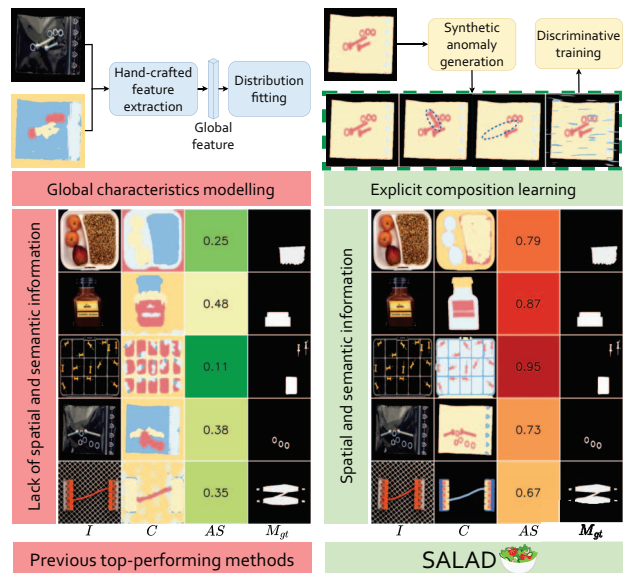
Figure 1. While previous approaches rely on handcrafted features, SALAD explicitly models the composition distribution by training directly on the composition maps C . SALAD is trained on simulated anomalous examples that are enclosed by a green dashed rectangle, whereas individual synthetic logical anomalies are highlighted with blue ellipses. SALAD improves the estimated anomaly scores (AS) on near-in-distribution logical anomalies.
