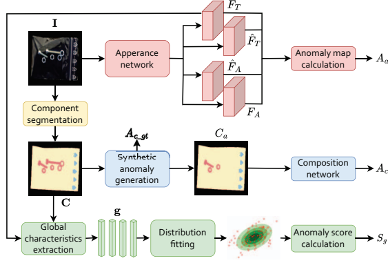
Figure 2. SALAD is constructed from a local appearance branch , a composition branch , and a global branch . Each branch focuses on a different level of image semantics. Synthetic anomalies are generated to train the composition branch. Composition maps are segmented using a component segmentation network .
