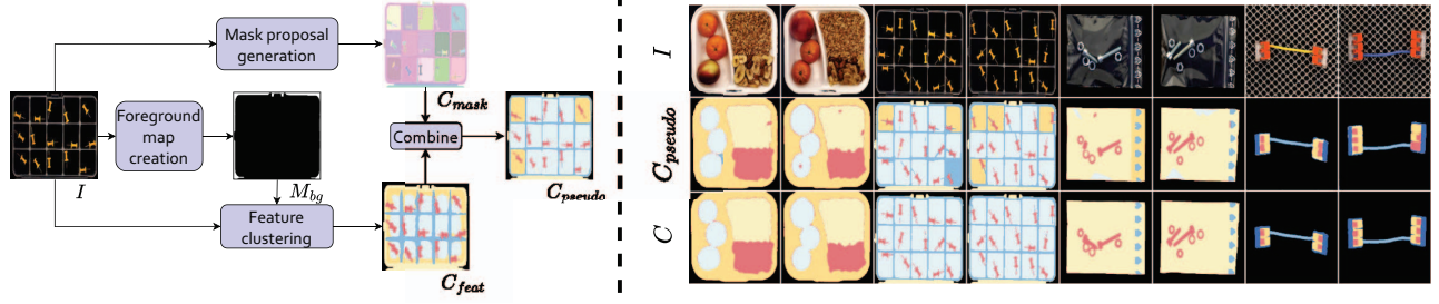
Figure 4. Left: Pseudo label C_{pseudo} generation procedure. The main idea is to combine precise mask generation from SAM-HQ [18] and the discriminative power from DINO [6]. Right: Comparisons of the final object composition maps C (generated by the composition segmentation model ) and the pseudo labels C_{pseudo} . Input images I are also depicted for comparison. Final object composition maps C contain less misclassified components than the pseudo labels C_{pseudo} .
