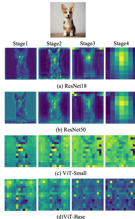
Figure 1. Significant feature gaps among heterogeneous models. For example, (a) CNN-based models [8] and (c) ViT-based models [6] have different features in different stages caused by different inductive biases and module functions.
