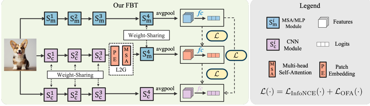
Figure 3. Overall. Firstly, our FBT fuses heterogeneous knowledge by merging the first three stages of CNNs, a projector L2G, and the last stage of MSAs/MLPs into the fused model. The fused model is adaptive and can be adjusted automatically according to different T.-S. pairs. Secondly, supervised by spatial-agnostic INFONCE loss [9] and target-wise OFA loss [7], the knowledge is transferred from the teacher to the fused model and student. All models are split into four stages following [7].
