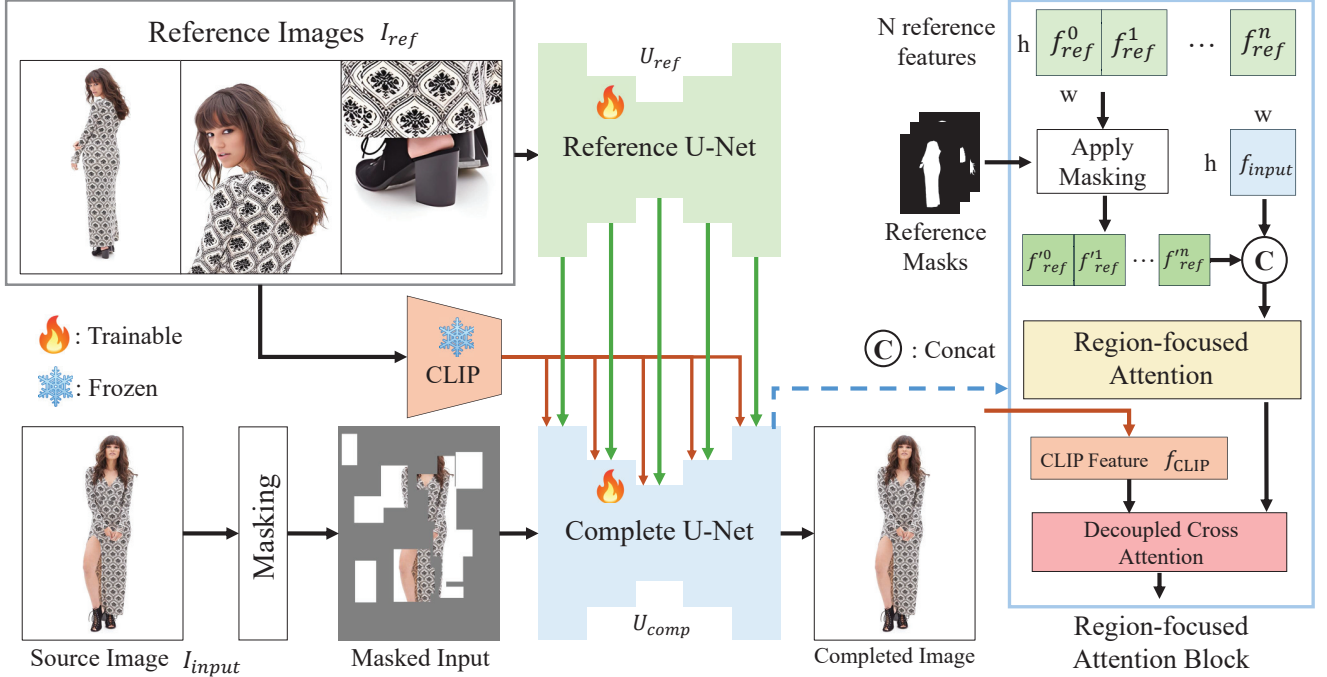
Figure 2. CompleteMe Pipeline. Our proposed CompleteMe utilizes a dual U-Net framework composed of a Reference U-Net ( U_{ref} ) and a Complete U-Net ( U_{comp} ). Given an input image ( I_{input} ) with masked regions, we first encode the input image to latent feature f_{input} . The Reference U-Net then extracts detailed visual features ( f_{ref}^0, f_{ref}^1, \dots, f_{ref}^n ) from multiple reference images ( I_{ref} ), which consist of different human body parts. Along with global semantic features ( f_{CLIP} ) extracted by CLIP, the reference features are processed within our novel Region-focused Attention (RFA) Block embedded in the Complete U-Net. These reference features are then explicitly masked according to reference masks, producing masked reference features ( f'_{ref}^0, f'_{ref}^1, \dots, f'_{ref}^n ). This explicit masking and concatenation strategy enables the model to precisely zoom in and focus on relevant human regions, establishing accurate and fine-grained correspondences through the Region-focused Attention mechanism. Finally, decoupled cross-attention integrates these refined local features with the global semantic CLIP features ( f_{CLIP} ), resulting in a detailed and semantically coherent completion.
