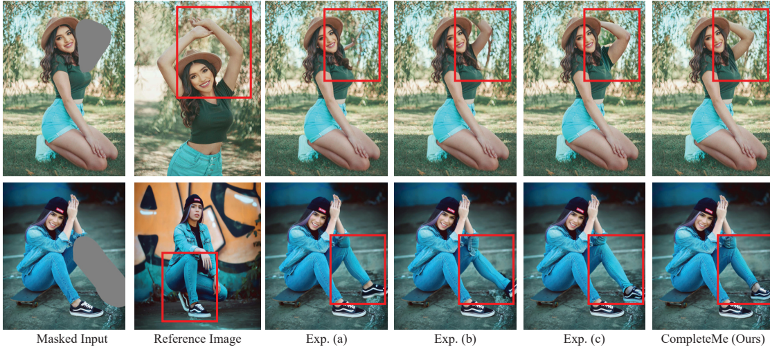
Figure 6. Qualitative Comparison on Different Training Strategies. The experimental index follows configurations in Table 5. The Red box highlights the finely detailed regions where different models exhibit varying performance based on distinct training strategies.
