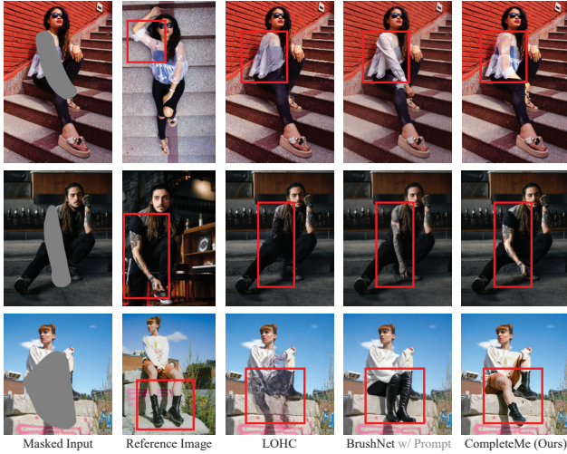
Figure 3. Qualitative Comparison with Non-reference Methods. We compare CompleteMe with non-reference methods, LOHC[43] and BrushNet [12]. Given masked inputs, these non-reference methods generate plausible content for the masked regions using image priors or text prompts. However, as indicated in the Red box , they cannot reproduce specific details such as tattoos or unique clothing patterns, as they lack reference images to guide the reconstruction of identical information.
