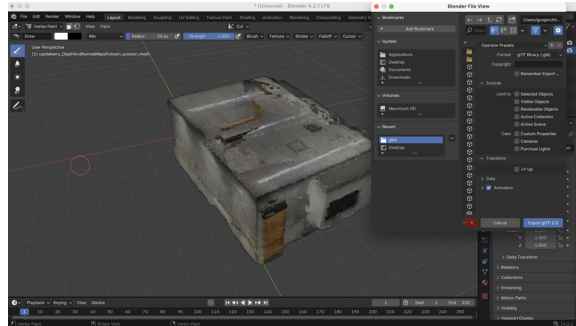
Figure 18. Converting the .ply files generated by DN-Splatter [49] to .gltf files using Blender. Transform +Y Up is kept unchecked following conventions of Habitat-Sim [39].
