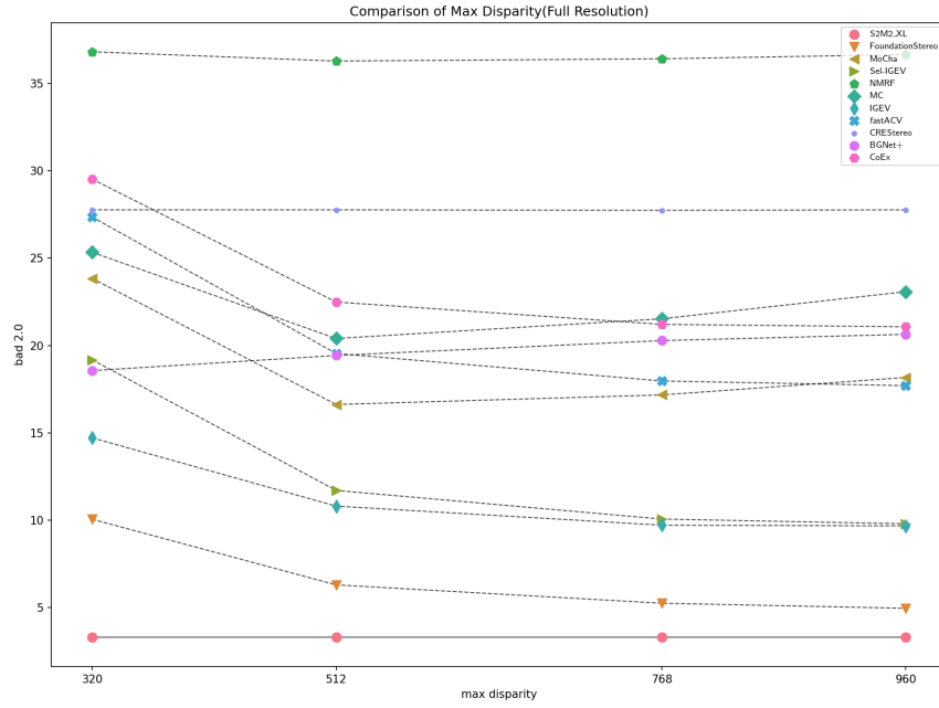
Figure 8. Performance comparison across four maximum disparity ( D_{max} ) settings at full resolution. The solid line indicates our S 2 M 2 model, which is unaffected by this parameter and included for reference.
