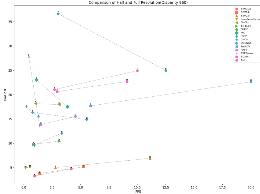
Figure 7. Accuracy vs. inference speed comparison between full (F) and half (H) resolution, with the maximum disparity set to 960. Inference speed was measured with float16 precision using PyTorch’s Automatic Mixed Precision (AMP).
