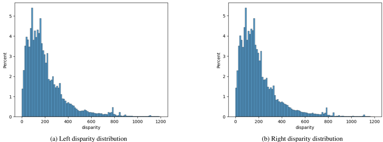
Figure 3. Benchmark dataset disparity distribution (x-axis: disparity (pixels), y-axis: proportion of the total dataset (%)): The figure illustrates the disparity distribution when the maximum disparity is set to 1200 pixels, covering 99.591% of the entire benchmark dataset.
