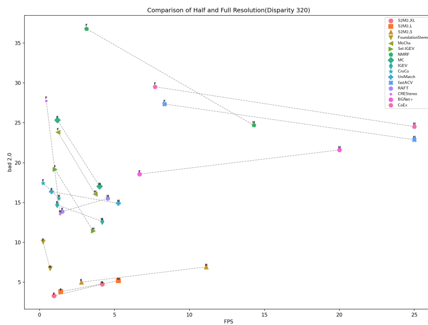
Figure 6. Accuracy vs. inference speed comparison between full (F) and half (H) resolution, with the maximum disparity set to 320. Inference speed was measured with float16 precision using PyTorch's Automatic Mixed Precision (AMP).
