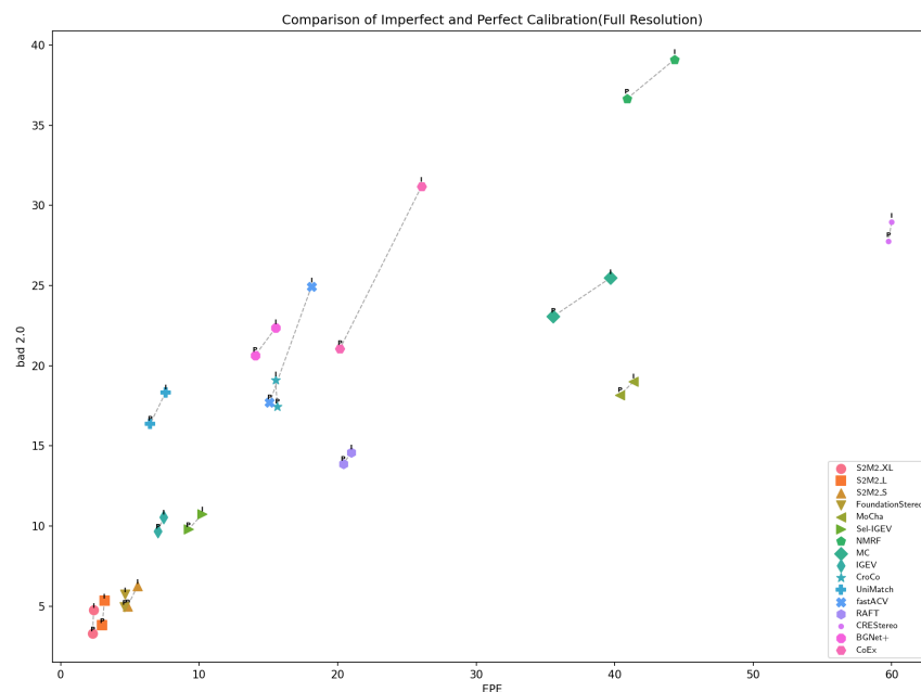
Figure 5. Comparison of model performance under perfect (P) and imperfect (I) calibration settings.
