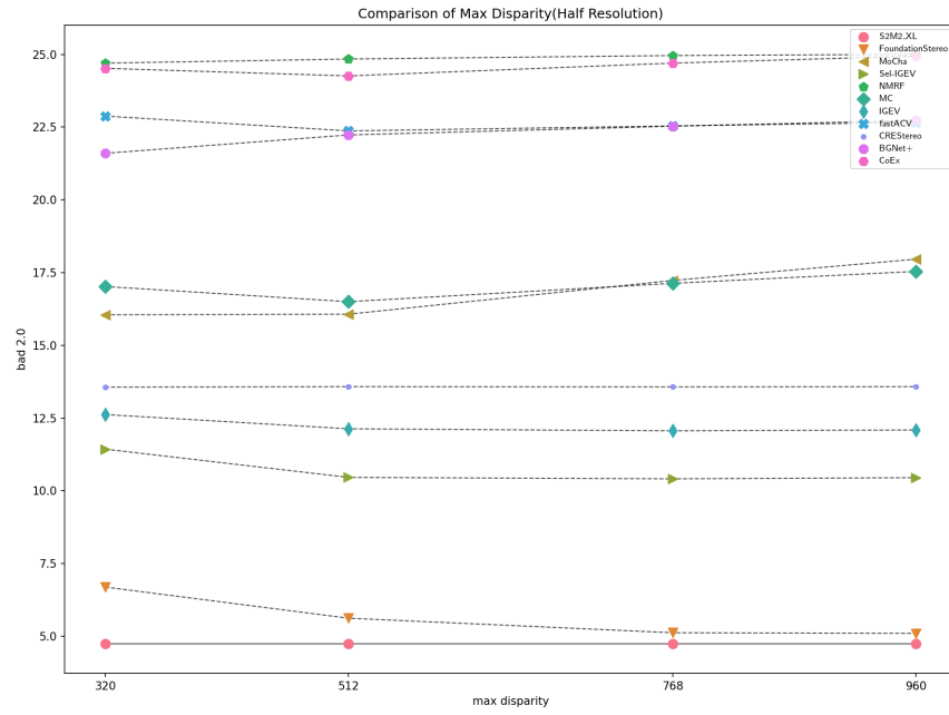
Figure 9. Performance comparison across four maximum disparity ( D_{max} ) settings at half resolution. The solid line indicates our S²M² model, which is unaffected by this parameter and included for reference.
