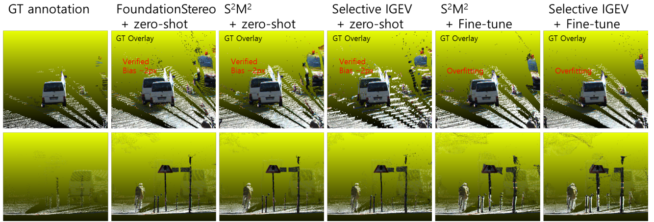
Figure 4. Qualitative comparison illustrating the negative effects of fine-tuning on a KITTI 2015 sample. Top row: Focuses on a vehicle area to highlight the bias between the zero-shot and fine-tuned models. The ground truth annotation from the training data is overlaid to visualize how the fine-tuned model adapts to the noisy label. Bottom row: Shows a pillar structure where the fine-tuned model estimates the pillar to be significantly thicker than its actual structure, a distortion not present in the zero-shot output.
