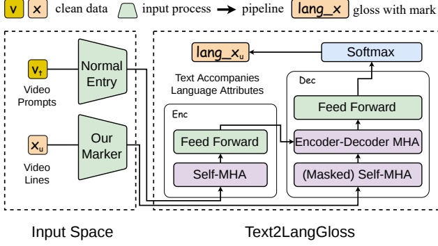
Figure 6. We enhance Text2Gloss [71] with a marker to generate the Gloss with linguistic properties. The v_t ( \mathbf{v}_t ) and x_u ( \mathbf{x}_u ) represent data types and abstract representations.
