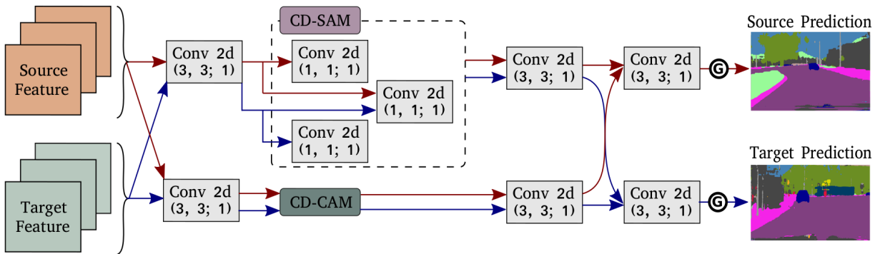
Figure 1: The network architecture of two cross-domain attention modules, where Conv 2d ( k, k; j ) indicates the 2D convolution with kernel size ( k \times k ) and stride j . The red and blue lines denote features from source and target domains, respectively.
