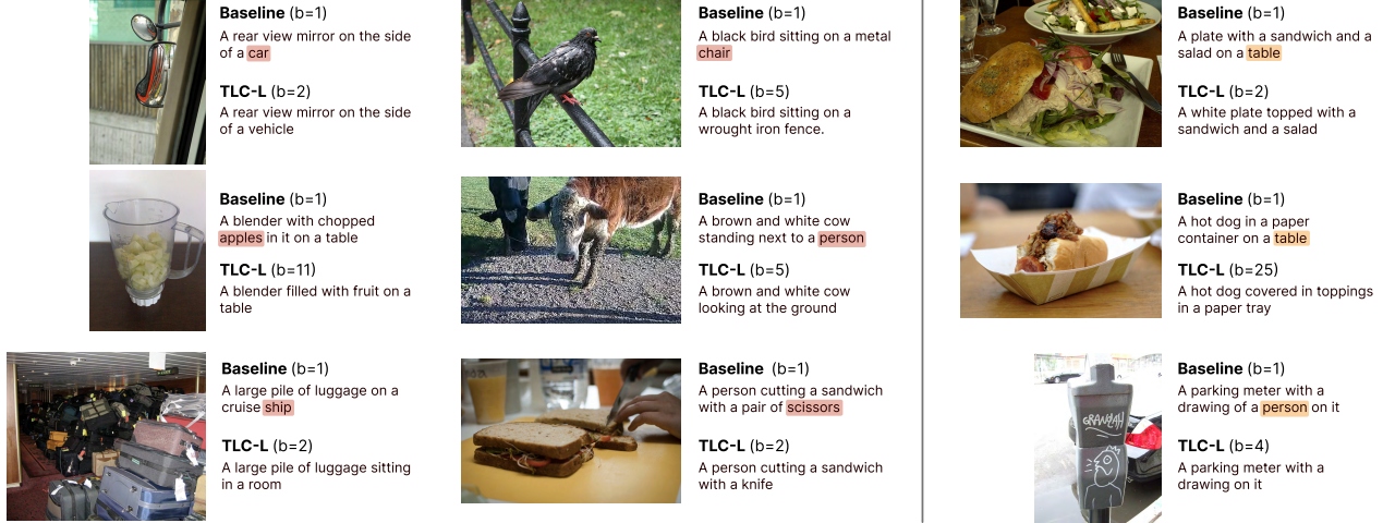
Figure 3. Qualitative examples from our test set in which TLC-L avoided hallucinations in the original (Baseline) captions. In the rightmost column, we show cases where the MS COCO object annotations did not exhaustively include all objects present. Captions are generated with OFA Large and a beam size of 25, and ( b = i ) refers to the index i of the beam as ranked by the Baseline.
