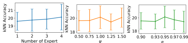
Figure 6. Sensitivity experiments of various hyperparameters in EVOLVE, tested on BYOL and Seq-imb Stream-51 streams.
