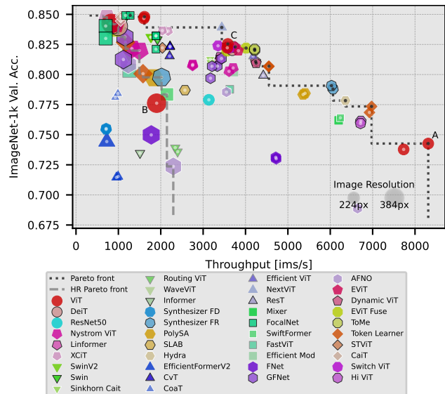
Figure 1. Pareto front (dotted line) showing the throughput-accuracy trade-off for efficient Vision Transformers. Markers (varying in shape and hue) represent different efficiency strategies, with black dots highlighting Pareto optimal models. Marker size indicates fine-tuning resolution. Baselines ViT-Ti@224 (A), ViT-Ti@384 (B), and ViT-S@224 (C) are shown, along with the Pareto front for high-resolution images (dashed line).
