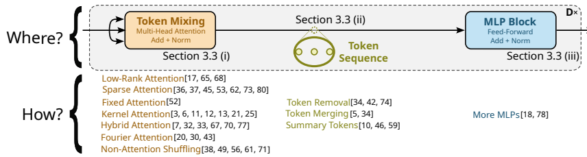
Figure 2. List of efficient Transformers (citation key in brackets) categorized at two levels: 1. Where does the approach change ViT? 2. How does the approach change ViT?
