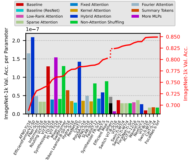
Figure 3. Accuracy (red line, right y-axis) and accuracy per parameter (bars, left y-axis) of models ordered by accuracy at a resolution of 224px. 14 of 47 models of intermediate size are grouped into others . See the supplementary material for the full plot.
