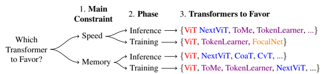
Figure 6. Suggestions on Which Transformer to Favor in image classification. First, choose the main constraint (1.), speed, or memory, and the phase you want to optimize this constraint at (2.): Inference or training. Based on that, we provide recommendations on which transformer to favor (3.) from the taxonomy classes of Baseline , Sequence Reduction , Hybrid Attention , Non-Attention Shuffling and Sparse Attention . See the supplementary material for a full list of Pareto optimal models for each metric.
