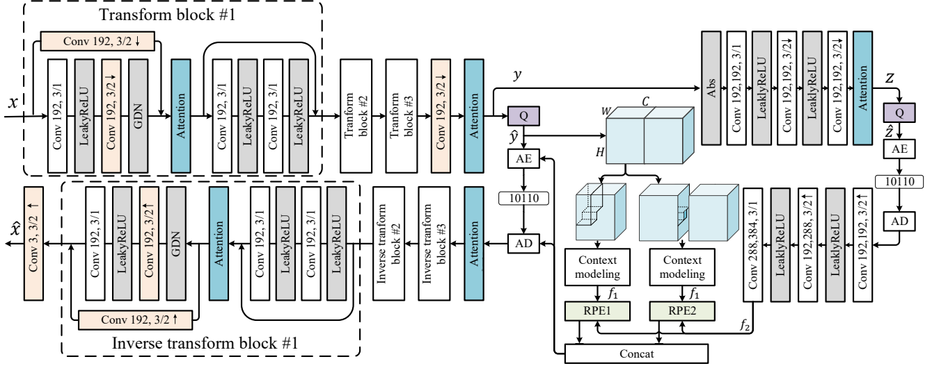
Figure 1: The overall framework of our image compression model. The context entropy model is a 3-D version.
