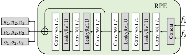
Figure 2: Residual parameter estimation module. There is only one residual connection and thus the RPE module is relatively light-weighted but effective.
