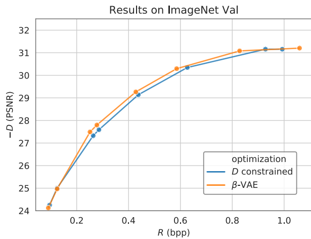
Figure A.2: Rate / PSNR performance for D constrained optimization and \beta -VAE.
