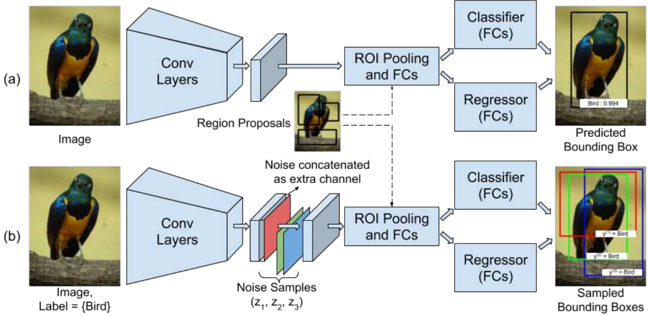
Figure 1. The overall architecture. (a) Prediction Network: a standard Fast-RCNN architecture is used to model the prediction net. For an input image, bounding box proposals are generated from selective search [35]. Features from each of these proposals are computed by the region of interest (ROI) pooling layers, which are then passed through the classifier and regressor to predict the final bounding box. (b) Conditional Network: a modified Fast-RCNN architecture is used to model the conditional net. For a single input image \mathbf{x} and three different noise samples \{\mathbf{z}_1, \mathbf{z}_2, \mathbf{z}_3\} (represented as red, green and blue matrix), three different bounding boxes \{\mathbf{y}^{(1)}, \mathbf{y}^{(2)}, \mathbf{y}^{(3)}\} are sampled for the given image-level label (bird in this example). Here the noise filter is concatenated as an extra channel to the final convolutional layer. For both the networks, the initial conv-layers are fixed during training. Best viewed in color.
