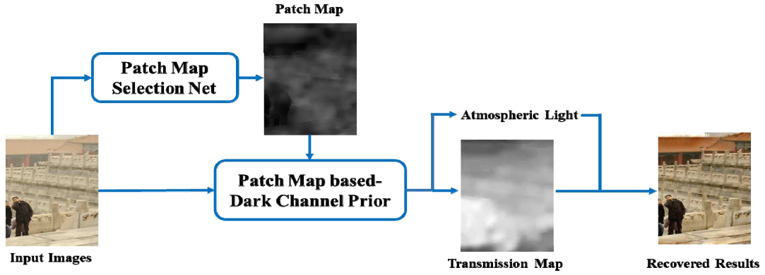
Figure 3: The flowchart of the proposed haze removal algorithm.
