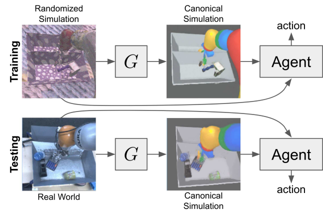
Figure 1: We learn a generator that translates randomized simulation images to a chosen canonical simulation version which are then used to train a robot grasping agent (top). The system can then be used to translate real-world images to canonical images, and consequently allow for Sim-to-Real transfer of the agent (bottom). Feeding both source and target images to the agent allows for joint finetuning of the agent in the real world.
