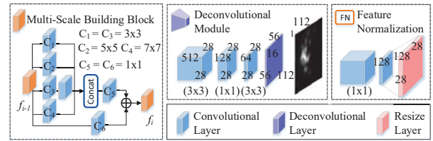
Figure 7. Components of the AG-CNN architecture.
