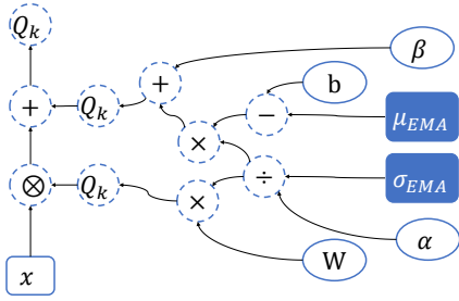
Figure 3: Stabilized batch norm folding: BN statistics \mu, \sigma and affine parameters \alpha, \beta are folded into parameters W and b of the preceding Conv or FC layers. Note that statistics \mu_{EMA} and \sigma_{EMA} from trained full-precision BN layers are used instead of per-batch statistics from quantized activations, to address the instability during quantization-aware fine-tuning.
