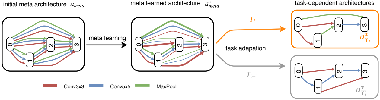
Figure 3: Conceptual illustration of the architectures at different stages of METANAS. Left: after initializing the one-shot model. Middle: meta-learned architecture. Right: architecture adapted to respective tasks based on meta-architecture. Colours of the edges (red, blue, green) denote different operations (Conv3x3, Conv5x5 and MaxPooling, respectively). Line-width of edges visualizes size of architectural weights \alpha (i.e., large line-width correspond to large \alpha values).
