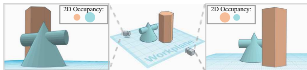
Figure 3. Toy example of 2D observations at different view angles of the same 3D scene. The number of occupied pixels/voxels of each instance (denoted as occupancy) is uncertain on 2D image, yet can be predicted robustly for the reconstructed 3D model.
