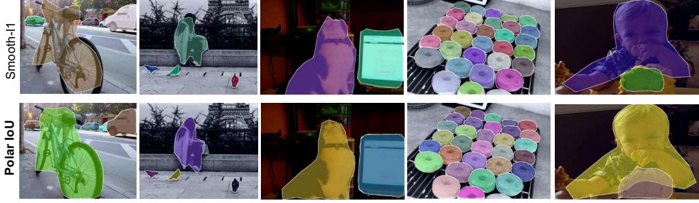
Figure 6 – Visualization of PolarMask with Smooth- l_1 loss and Polar IoU loss. Polar IoU Loss achieves to regress more accurate contour of instance while Smooth- l_1 Loss exhibits systematic artifacts.
