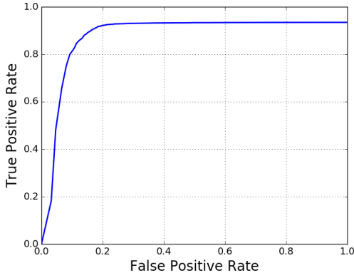
Fig. 7: ROC Curve at IOU Threshold of 0.5
