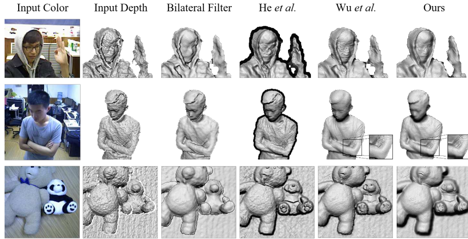
Fig. 8. Comparison of color-assisted depth map enhancement between bilateral filter, He et al. [15], Wu et al. [44] and our method. The closeup of the finger region demonstrates the effectiveness of unsupervised shading term in our refinement net loss.
