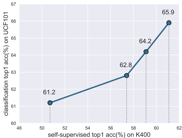
Figure 3: Relation between self-supervised accuracy and classification accuracy. Self-supervised model (DPC) is trained on K400 and the weights at epoch {13, 48, 81, 109} are saved, which achieve {50.7%, 57.4%, 59.1%, 61.1%} self-supervised accuracy respectively. The checkpoints are evaluated by finetuning on UCF101.
