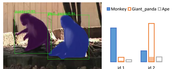
Figure 3. An example of class calibration. In this video, “monkey” is a reliable category while “giant panda”, “ape” are not reliable based on the average scores of all the object candidates in the video. Thus, the detection scores of the unreliable classes (“giant panda”, “ape”) are re-weighted with factor \beta .
