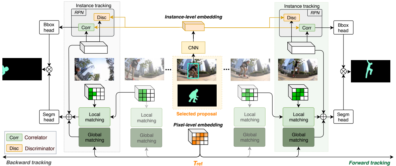
Figure 2. Details of the bi-directional Instance-Pixel Dual-Tracker (IPDT).
