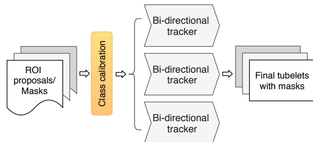
Figure 1. An overview of our framework. The proposals generated by Mask R-CNN [6] are first calibrated on the class prediction and then fed into the proposed bi-directional tracker IPDT. The final tubelets are filtered with post-processing.
