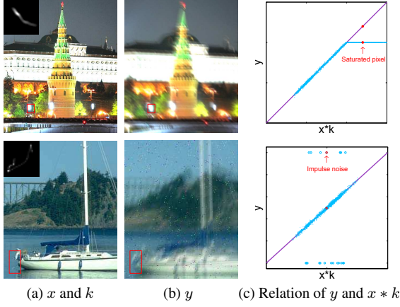
Figure 1. Properties of saturated pixels and impulse noise. (a) Clear images x with the blur kernels k . (b) Blurred images y with saturated pixels (top) and impulse noise (bottom). (c) Blue points: the relation between y and x * k . Purple lines: the ideal case of y = x * k .
