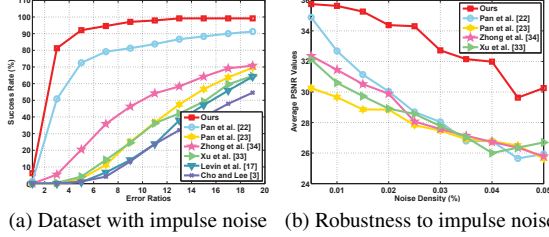
Figure 11. Quantitative evaluations on dataset with impulse noise. SNR than the others. The error ratio [16] is also used as the quality metric. As Figure 11(a) shows, our method performs favorably against the state-of-the-art methods.
