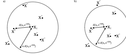
Figure 2. A simplified 2-dimensional projection of the neighbours for anchor \mathbf{x}_i , here \mathcal{S}_i contains two positive and four negative samples. Distance d(x, y) is squared Euclidean. a) The current \kappa and clustering of class y_i specify an exclusion boundary containing all negatives samples, as such none are currently deemed suitable for training. b) On a subsequent epoch a smaller \kappa and tighter class clustering now yields a negative sample outside the exclusion boundary. This negative and the positive sample further outside the exclusion boundary are used to complete a triplet that is guaranteed to violate the triplet constraint.
