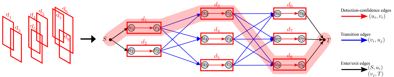
Figure 3: Over a set of prelabeled detections a min-cost flow network is defined. Each detection is represented by an observation edge with the confidence cost. ST-shortest paths are computed over this graph, red shadow.
