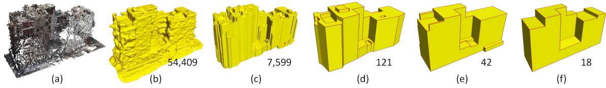
Figure 8. Comparison with four state-of-the-art methods on a building dataset. (a) Input point cloud. (b) Model reconstructed by the Poisson surface reconstruction algorithm [11]. (c) The result of the 2.5D Dual Contouring approach [27]. (d) The result of [15]. (e) The result of [16]. (f) Our result. The number under each sub-figure indicates the total number of faces in the corresponding model.
