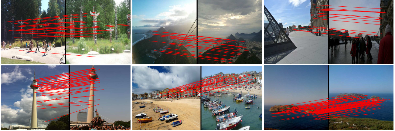
Figure 8: Visualization of feature correspondences between images in query and database using DELF+FT+ATT. For each pair, query and database images are presented side-by-side. DELF successfully matches landmarks and objects in challenging environment including partial occlusion, distracting objects, and background clutter. Both ends of the red lines denote the centers of matching features. Since the receptive fields are fairly large, the centers may be located outside landmark object areas. For the same queries, CONGAS fails to retrieve any image.
