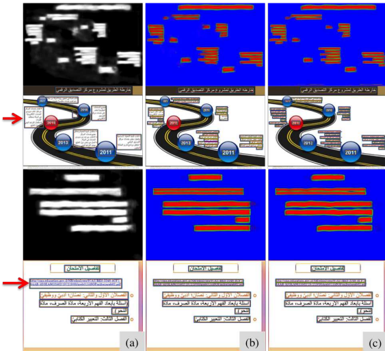
Figure 5. Effectiveness of the border class for text detection. (a), (b), and (c) are decoding results on the testing PPT dataset using models of single-res. w/o border, single-res. w/ border, and multi-res. w/ border, respectively. See differences in arrowed regions.
