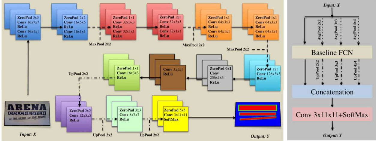
Figure 4. Fully convolutional networks used in the proposed method. Left: single resolution FCN. Right: multi-resolution FCN.
