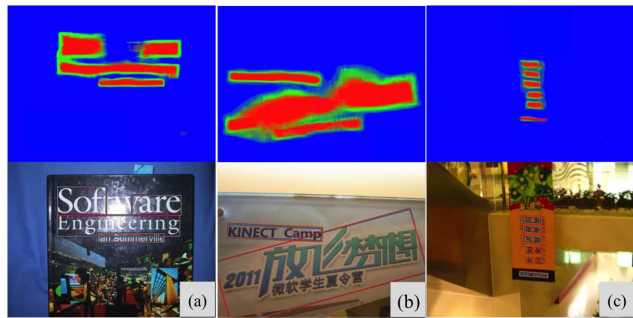
Figure 9. Failure cases. (a) over-segmentation; (b) under-segmentation; and (c) incorrect semantic grouping.
