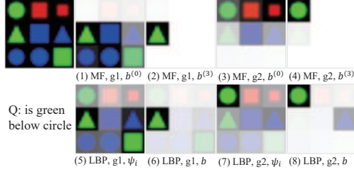
Figure 3: Visualization of MF-G2 and LBP-G2 on the test set of large. b^{(0)} or \psi_i represents the initial attention, b^{(3)} or b represents the refined attention after MF or LBP. The query looks for a green object under a circle.
