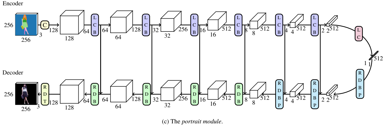
Figure 2: Full configuration of the CNN models presented in the main paper. Data size proportions scale logarithmically. Joining arrows indicate concatenation along the filter axis. The transformation blocks are: C 4 \times 4 convolution, LCB LReLU, 4 \times 4 convolution, batchnorm, F fully connected layer, DB 4 \times 4 deconvolution, batchnorm; RDB ReLU, 4 \times 4 deconvolution, batchnorm; D 4 \times 4 deconvolution; LC LReLU, 4 \times 4 convolution; RDBP ReLU, deconvolution, batchnorm, dropout; RDT ReLU, deconvolution, tanh. The portrait module can either be used with color maps as input as depicted here (3 channels) or with probability maps as input (22 channels).
