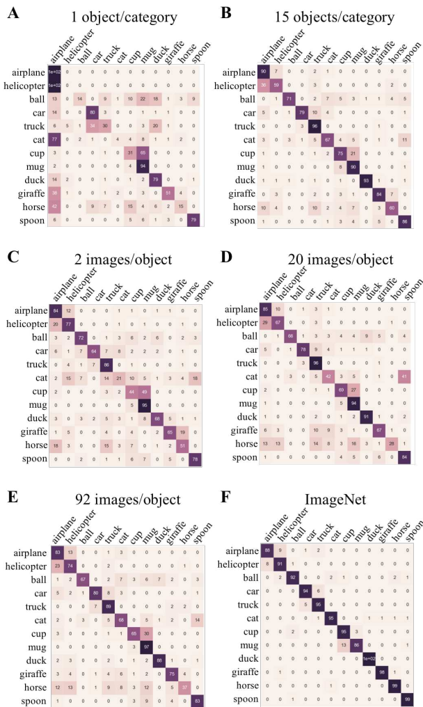
Figure 6. Confusion matrices showing the effects of increasing object diversity (A, B) or object view diversity (C, D, E), along with a comparison using ImageNet (F). Row labels are true categories and column labels are predictions.
