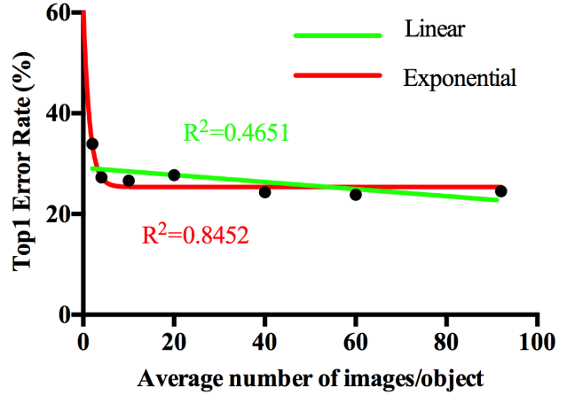
Figure 5. Experiment 2: Top-1 error rate on ImageNet test set as a function of object view diversity in EMMI training set, ranging from 2 to 92 images per object, with 12 objects per category. Total number of training images per category varies from 24 to 1100. (Random baseline error rate for 12 categories is \frac{11}{12} \approx 92\% .)
