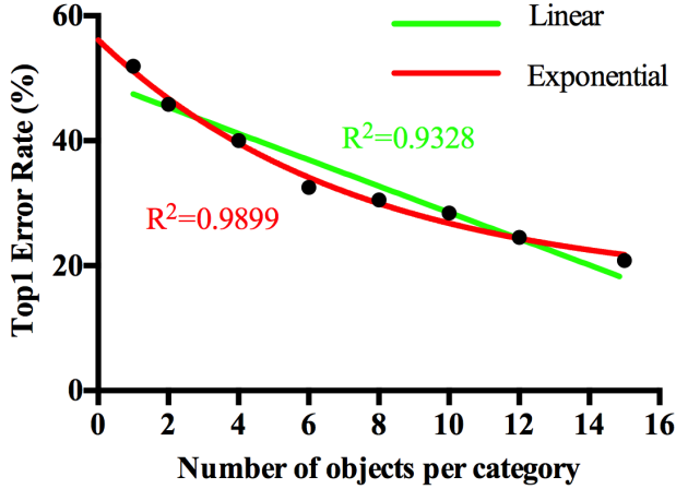
Figure 4. Experiment 1: Top-1 error rate on ImageNet test set as a function of object diversity in EMMI training set, ranging from 1 to 15 distinct physical objects per category, with total number of training images per category held constant at 1100. (Random baseline error rate for 12 categories is \frac{11}{12} \approx 92\% .)
