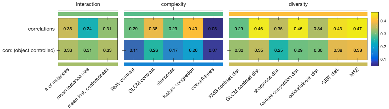
Figure 4: Correlations coefficients indicating how well various dataset qualities predict accuracy. The first row is based on all object×subject combinations while the second row only considers variations among subjects. See text for a description of each metric.
