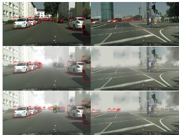
Figure 1. Examples of unrestricted object detection. The first row denotes the pictures from the Cityscapes [4], while pictures of the last two rows are detected from the Foggy Cityscapes [32]. The results of the first two rows are detected by the traditional Faster-RCNN [29] trained on Cityscapes, and we can see that many objects are missing on the domain shifted Foggy Cityscapes (the second row). The third row shows the results of our approach, and the domain disparity between two datasets can be effectively removed.
