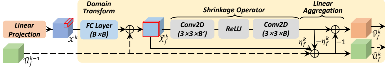
Figure 2. Data flow graph of our proposed Tensor ADMM-Net: (a) The general framework is constructed by connecting each Stage in a sequence order. In each Stage , multiple transformation Patterns are processed in parallel. (b) Details of each Pattern . The dashed line denotes the data flow between two consecutive stages while the solid line denotes the data flow inside the same stage.
