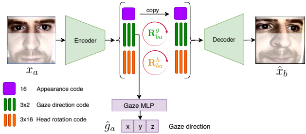
Figure 2: Disentangling appearance, gaze and head pose variations from an image with our Disentangling Transforming Encoder-Decoder (DT-ED). We learn to translate between pairs of images of the same person by rotating the gaze and head pose codes. The encoder-decoder are supervised by a pixel-wise L_1 loss (Eq. 3), with the gaze embedding additionally supervised via gaze regression (Eq. 5).
