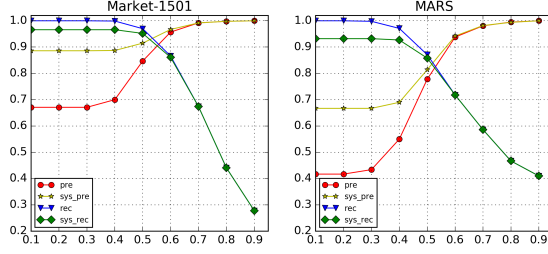
Figure 4: Precision scores and recall scores of different \lambda . In this figure, "pre" denotes the precision. "rec" denotes the recall. "sys_pre" and "sys_rec" respectively denote the precision and recall of using the symmetry condition. The horizontal axis is the value of the \lambda .
