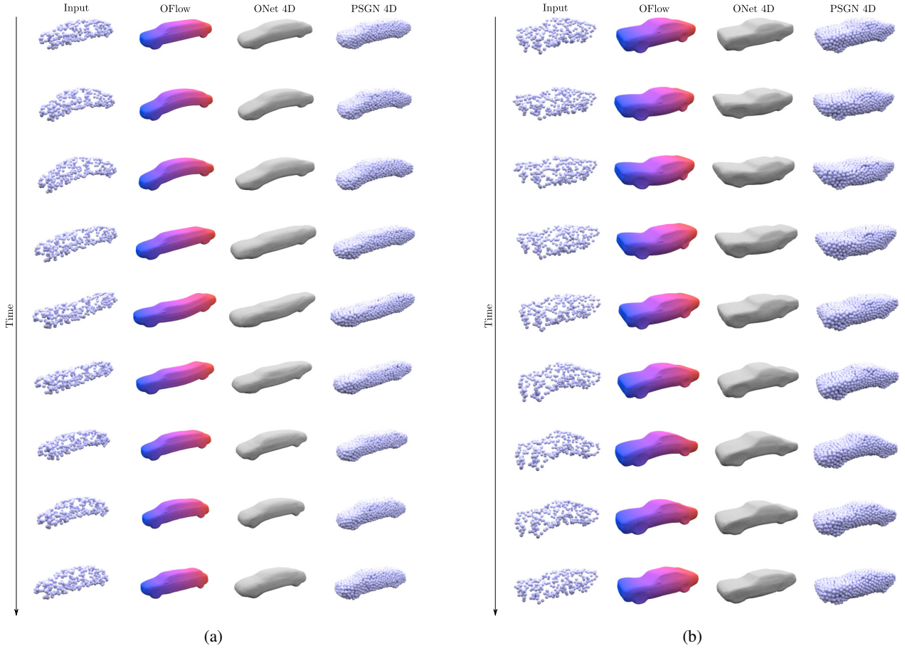
Figure 5: 4D Point Cloud Completion (Warping Cars) . This figure shows two examples from the test set of the point cloud completion experiment on the warping cars dataset. For both examples, we show the input as well the output of OFlow, ONet 4D, and PSGN 4D for 9 equally spaced time steps between 0 and 1.
