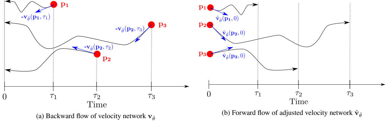
Figure 3: Batch Processing. The figure illustrates how we reformulate the backward flow of \mathbf{v}_{\hat{\theta}} as the forward flow of the adjusted velocity network \hat{\mathbf{v}}_{\hat{\theta}} (1) to perform batch processing of points \mathbf{p}_i with different time values \tau_i .
