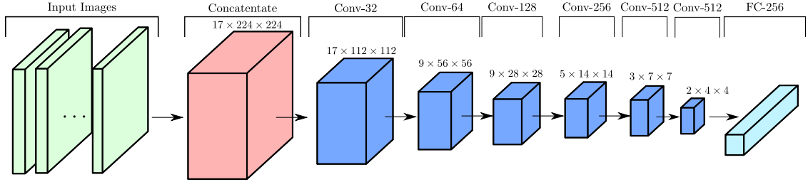
(b) 4D reconstruction from Image Sequences. The L = 17 input RGB images are concatenated to obtain a tensor of size 3 \times 17 \times 224 \times 224 . We pass the tensor through six convolutional layers which downsample the input while increasing the number of feature maps. The final feature vector is obtained by passing the output through a 256-dimensional fully connected layer.
