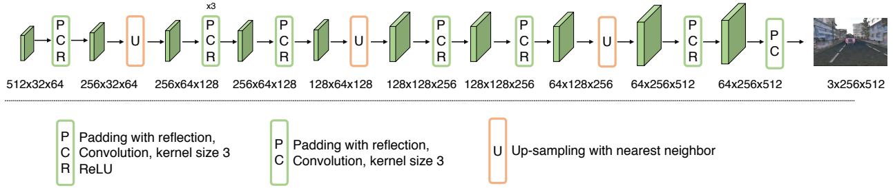
Figure 1: Architecture of the decoder.
