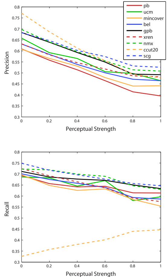
Figure 4. The optimal precision and recall values for all algorithms, benchmarked under different label strengths. By increasing the perceptual strength, we transform the problem from “boundary detection” to “strong boundary detection”. The precision values for algorithms dropped 28.7% in average. In contrast, the recall values, which are not affected by the precision bonus, only dropped 9% in average.
