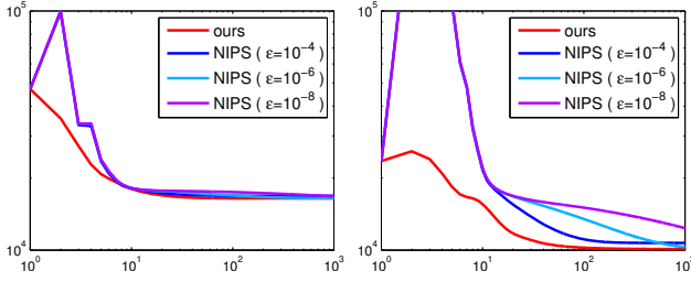
Figure 4. Left to right: Comparison of the energy decrease for the non-convex log TV and TGV between our method and NIPS [25]. Our proposed algorithm achieves a lower energy in the limit and drops the energy much faster in the beginning.
