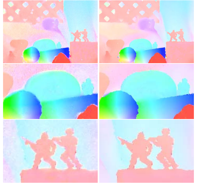
Figure 6. Comparison between TGV ( left ) and non-convex TGV ( right ) for the image pair Army from the Middlebury Optical Flow benchmark [1] and two zooms. The TGV is obtained with \lambda = 50 , \gamma = 0.04 , \alpha_1 = 0.5 , \alpha_2 = 1.0 and the result with non-convex TGV using p = 1/2 , \lambda = 40 , \gamma = 0.04 , \alpha_1 = 0.5 , \alpha_2 = 1.0 .
