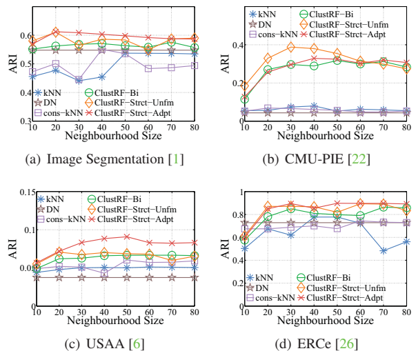
Figure 5. ARI curve: comparison between different methods on the spectral clustering performance given different scales of neighbourhood k . The neighbourhood size M used on computing the adaptive Gaussian kernel size is fixed to 20.
