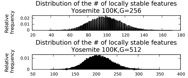
Figure 5. Histograms of descriptor dimensionality after the online selection of locally optimized tests. G denotes the dimensionality of the globally optimized feature set.
