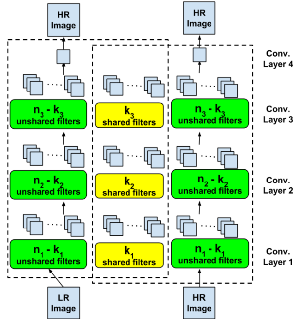
Figure 4. The Partially Coupled SR Networks (PCSRN), as the pre-training part of Model IV. Note it does not contain the fully-connected recognition sub-networks. For each channel, its recognition sub-network is the same as in Fig. 1 (fc4, fc5 and softmax). The two channels share k_i convolutional filters in the i -th layer.
