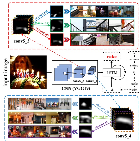
Figure 1. The illustration of channel-wise visual attention in two convolutional layers ( conv5\_3 and conv5\_4 in VGG19) when predicting cake from the captioning a woman sitting at a table with cake. At each layer, top 3 attentive channels are visualized by showing the 5 most responsive receptive fields in the corresponding feature maps [40].
