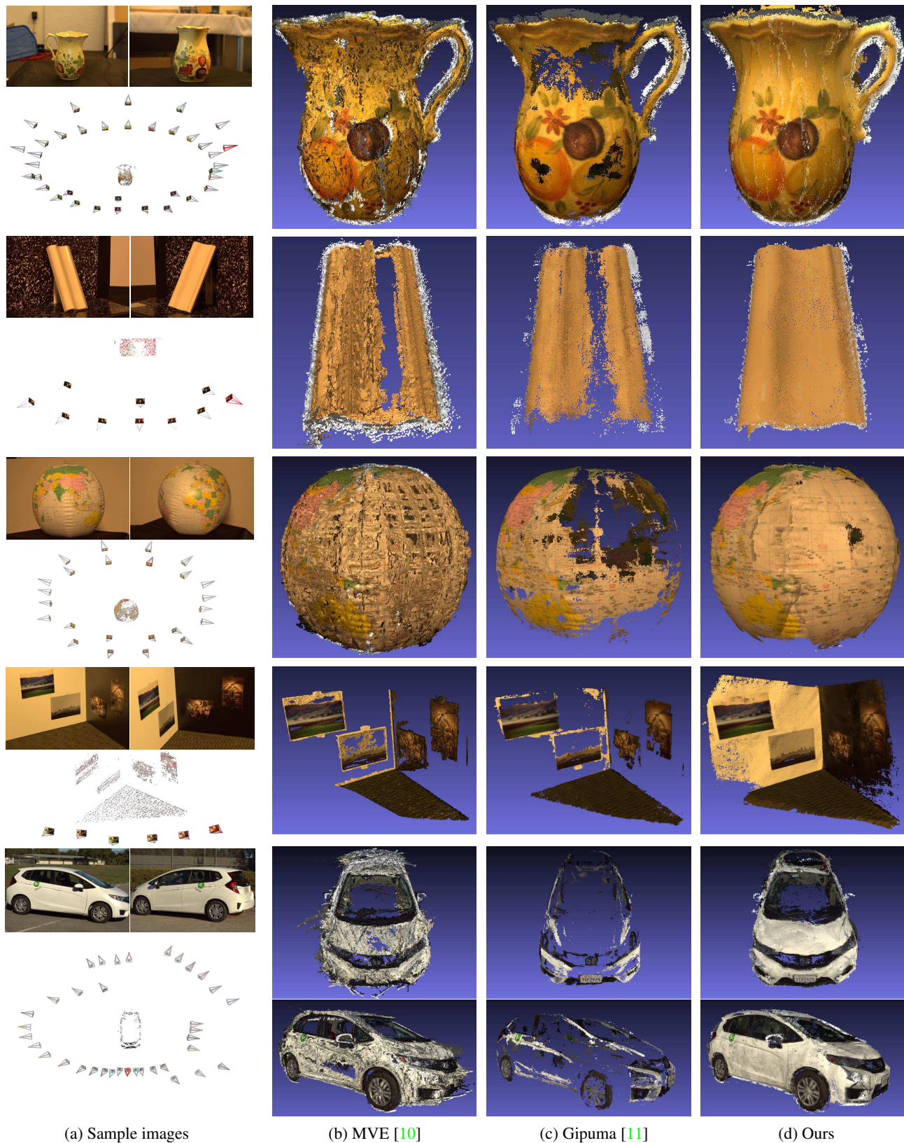
Figure 9: Comparison with state-of-the-art MVS methods [10, 11] for complete reconstruction. From top to bottom rows: VASE (36 views), TILE (10 views), BALLOON (24 views), CORNER (6 views), and CAR (36 views).
