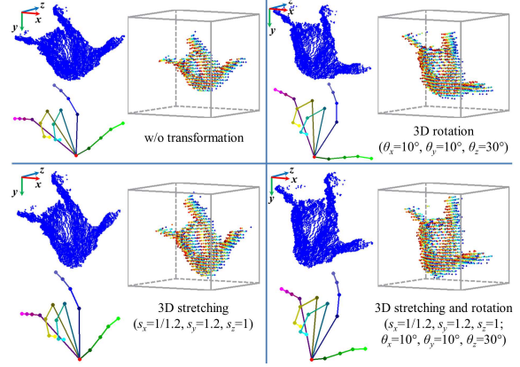
Figure 4: An example of 3D data augmentation. Top-left : original point cloud, ground truth and TSDF volume. Bottom-left : point cloud, ground truth and TSDF volume after 3D stretching. Top-right : point cloud, ground truth and TSDF volume after 3D rotation. Bottom-right : point cloud, ground truth and TSDF volume after 3D stretching and rotation. For illustration purpose, we only draw the projective D-TSDF volume on z direction.
